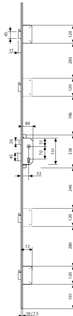
TLPN3 / TLPS3 / TLPF
